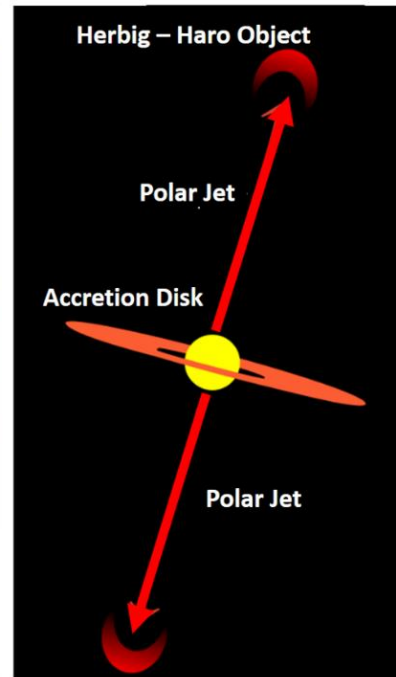
Abstract Structure of a Herbig – Haro Object
